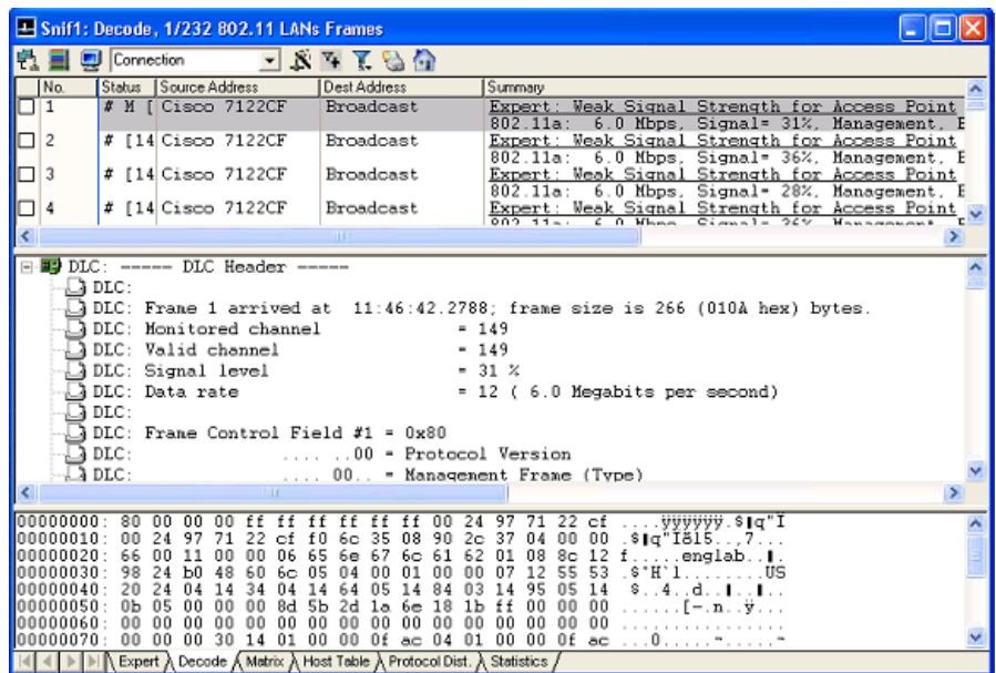
Fig 2: Sniffer Portable Professional decode view shows the results of a protocol analysis by displaying packets in three color-coded viewing panes: summary, detail, and hex codes.
